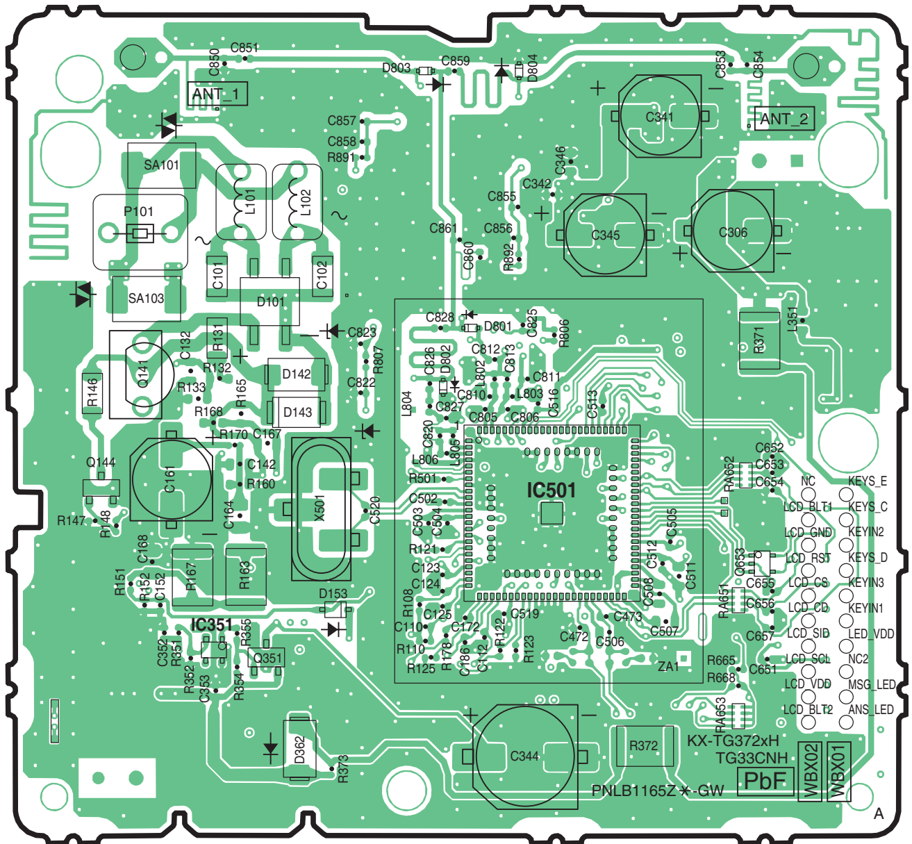
KX-TG3721/3722 CIRCUIT BOARD (Base Unit_Main (Component View))
