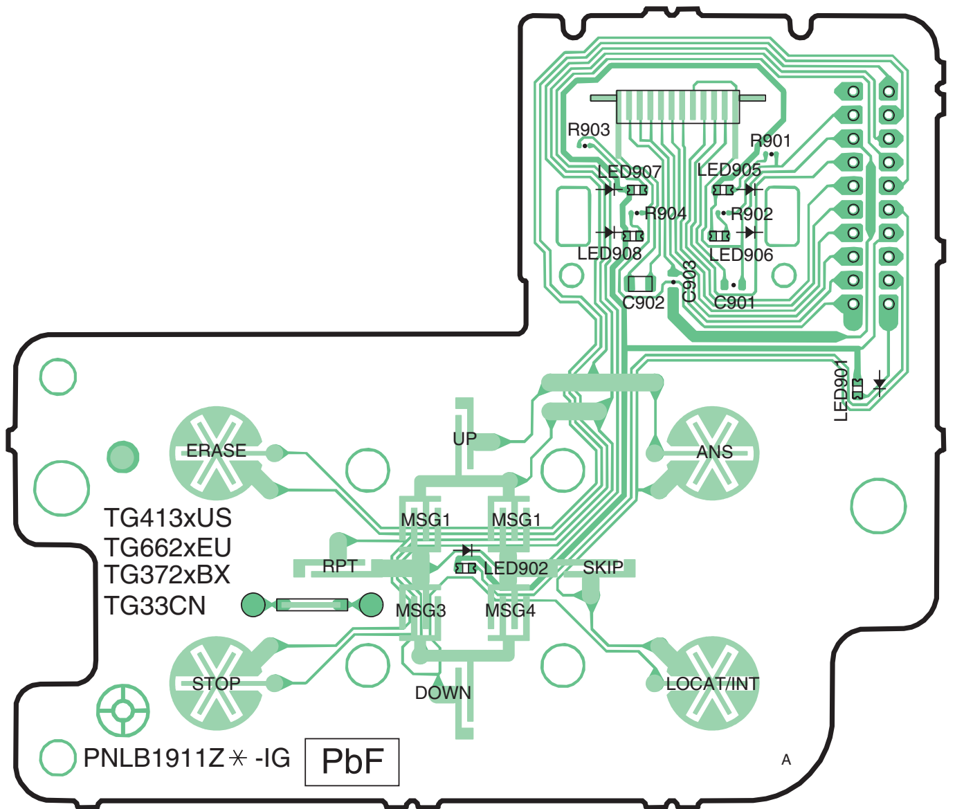
KX-TG3721/3722 CIRCUIT BOARD (Base Unit_Operation (Component View))
